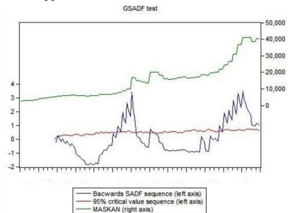
Figure 2. The GSADF test for detecting multiple bubbles
